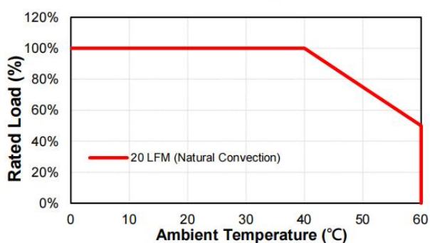
QXP-PAD Derating Curve
